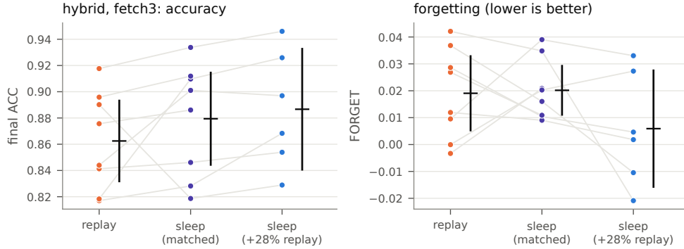
Figure 4: SNN+Transformer agent, fetch3: replay, sleep with its replay budget matched exactly to the same-seed replay run, and the original sleep runs, which consumed 28% more replayed states. Lines connect the same seed; bars are means with 95% CIs.
