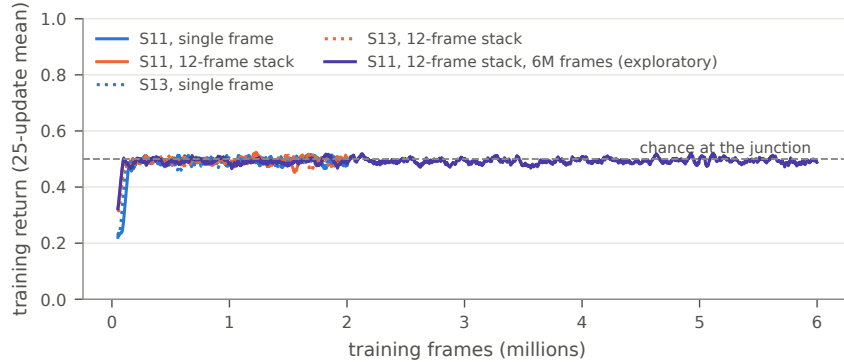
Figure 6: Memory-benchmark probes (CNN, one seed each, learning rate 0.0003): training return on MiniGrid-MemoryS11 and S13 with a single frame or a stack of the last 12 frames. Every run stays at chance.
