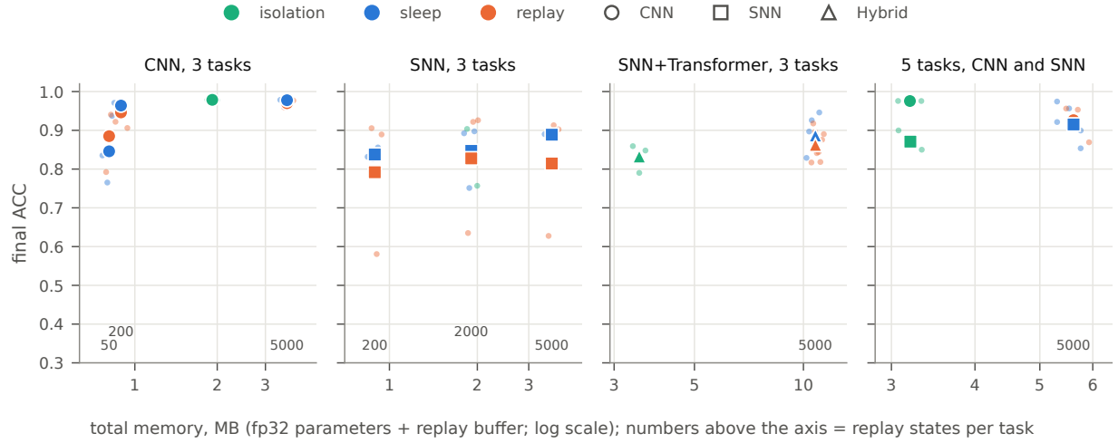
Figure 5: Final ACC against total memory (fp32 parameters plus replay buffer, log scale). Small dots: seeds; large markers: means. Numbers above the axis: replay states stored per task. 5-task SNN runs use the fair budget of 450k frames per task (see Section 6).
