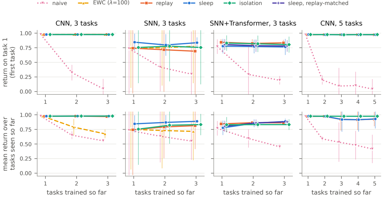
Figure 3: Forgetting curves. Top: return on the first task after each training stage; bottom: mean return over the tasks seen so far. Mean over seeds with 95% CIs (3 seeds per arm, except the SNN+Transformer agent: replay 8, replay-matched sleep 8, sleep 6). Methods are slightly offset horizontally so that overlapping lines stay visible.
