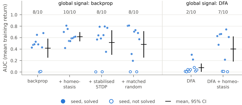
Figure 2: DoorKey-6x6, 400k frames, 10 seeds per arm. Dots: seeds (filled = solved, i.e. final return above 0.5); bar: mean and 95% CI of the AUC; numbers: solve counts.
