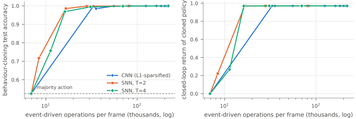
Figure 1: Operation-count frontier (behaviour cloning of a DoorKey-6x6 teacher, 2 seeds per point). Each point is one activity-penalty setting. Left: held-out action accuracy; right: closed-loop return of the cloned policy. The dashed line is the majority-action accuracy.
