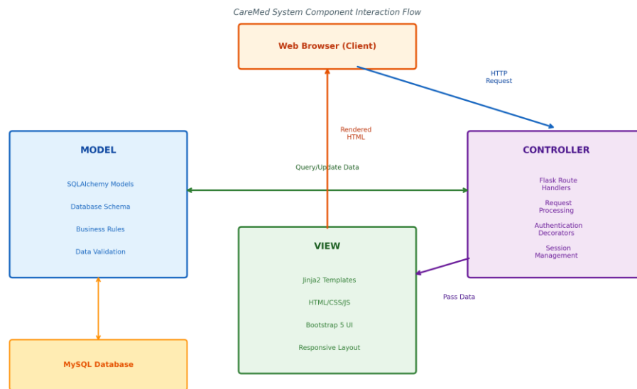
Figure 7. Model-View-Controller (MVC) Architecture Pattern
