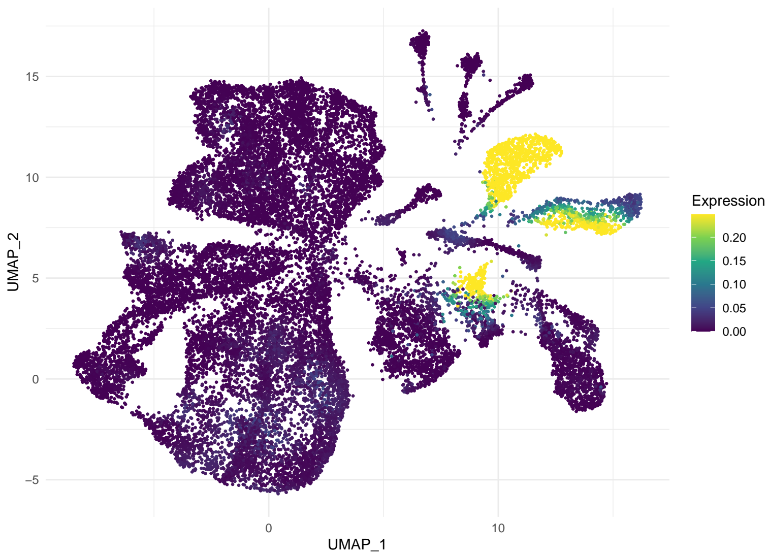
FGF7 (MAGIC smoothed)
