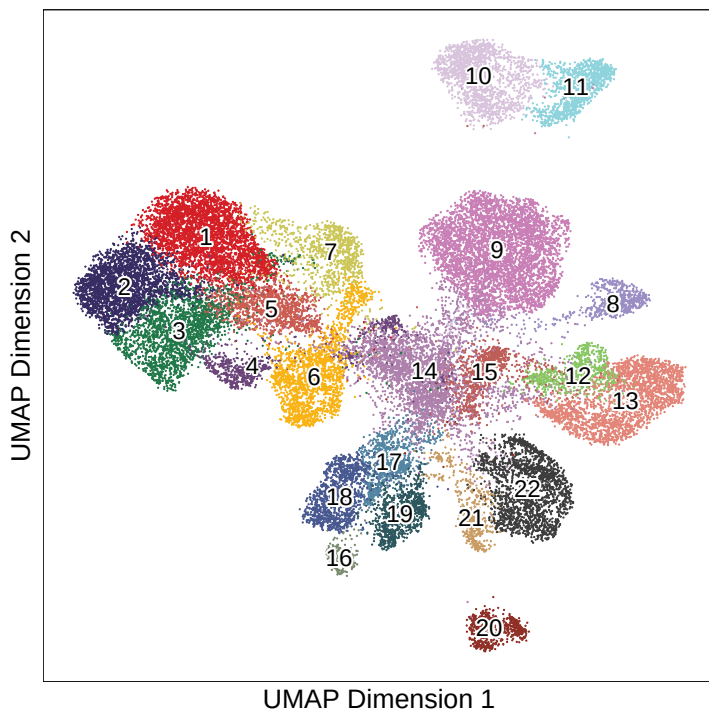
UMAP of Harmony colored by colData : Clusters
