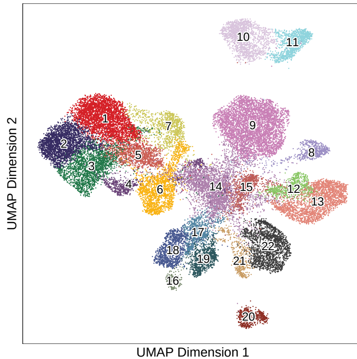
All Clusters
