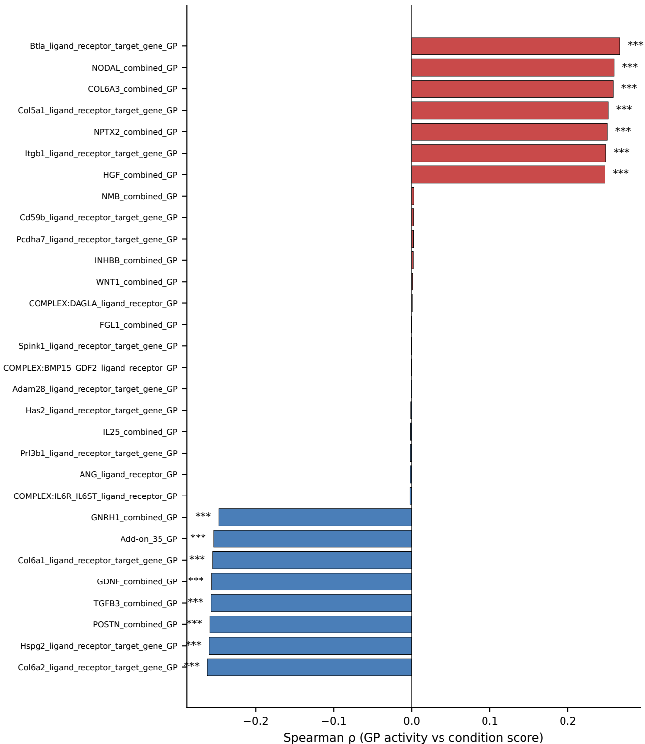
Condition-associated gene programs (per-cell \rho ; stars FDR; exploratory)
