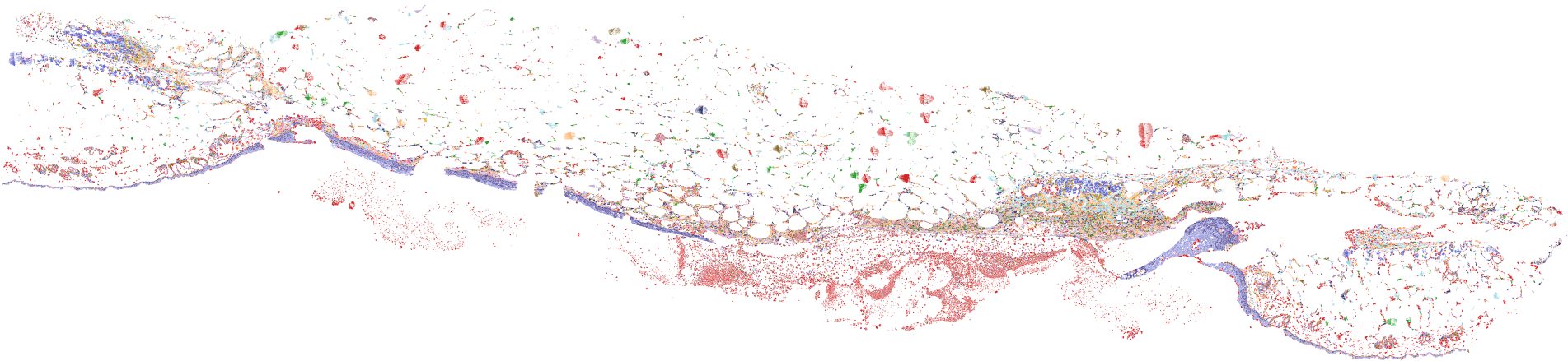
XE793-D – Predicted Cell Types
