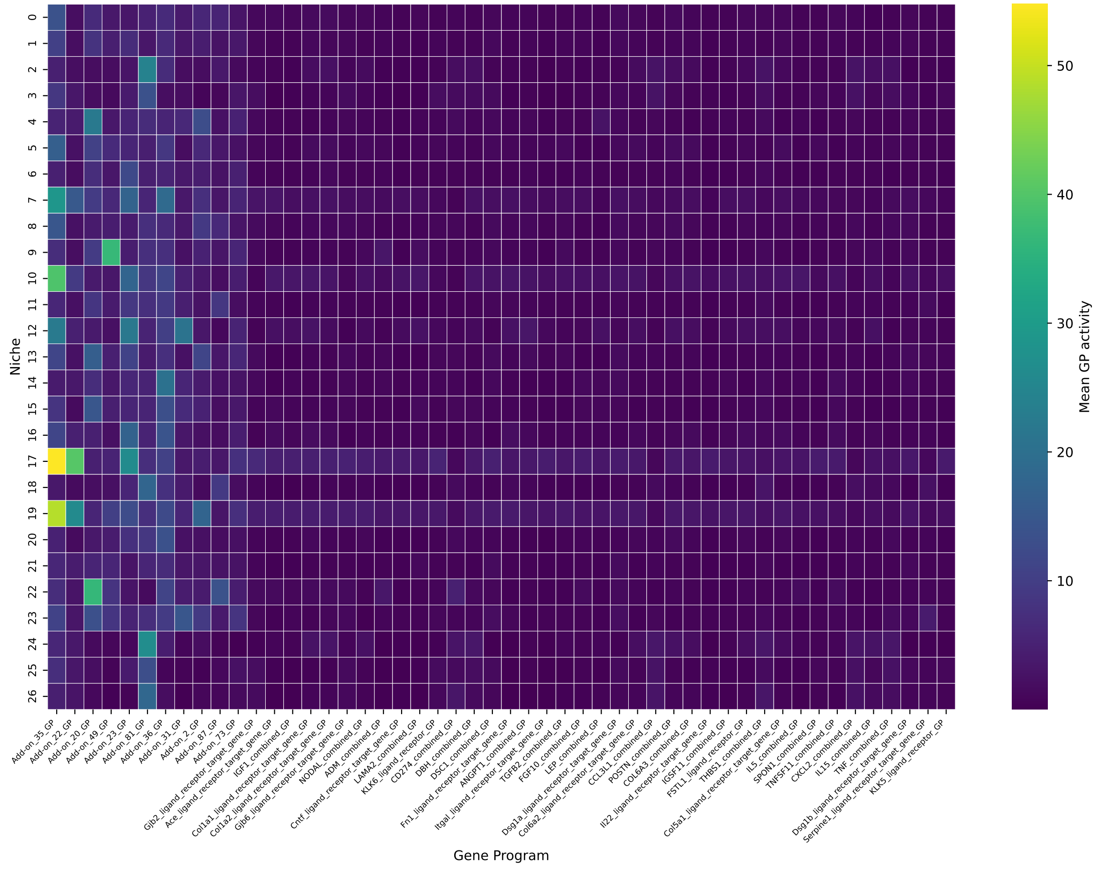
Top variable gene programs across niches
