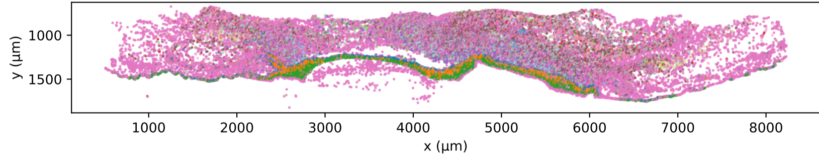
XE766-L (lesion) — Cell Types
