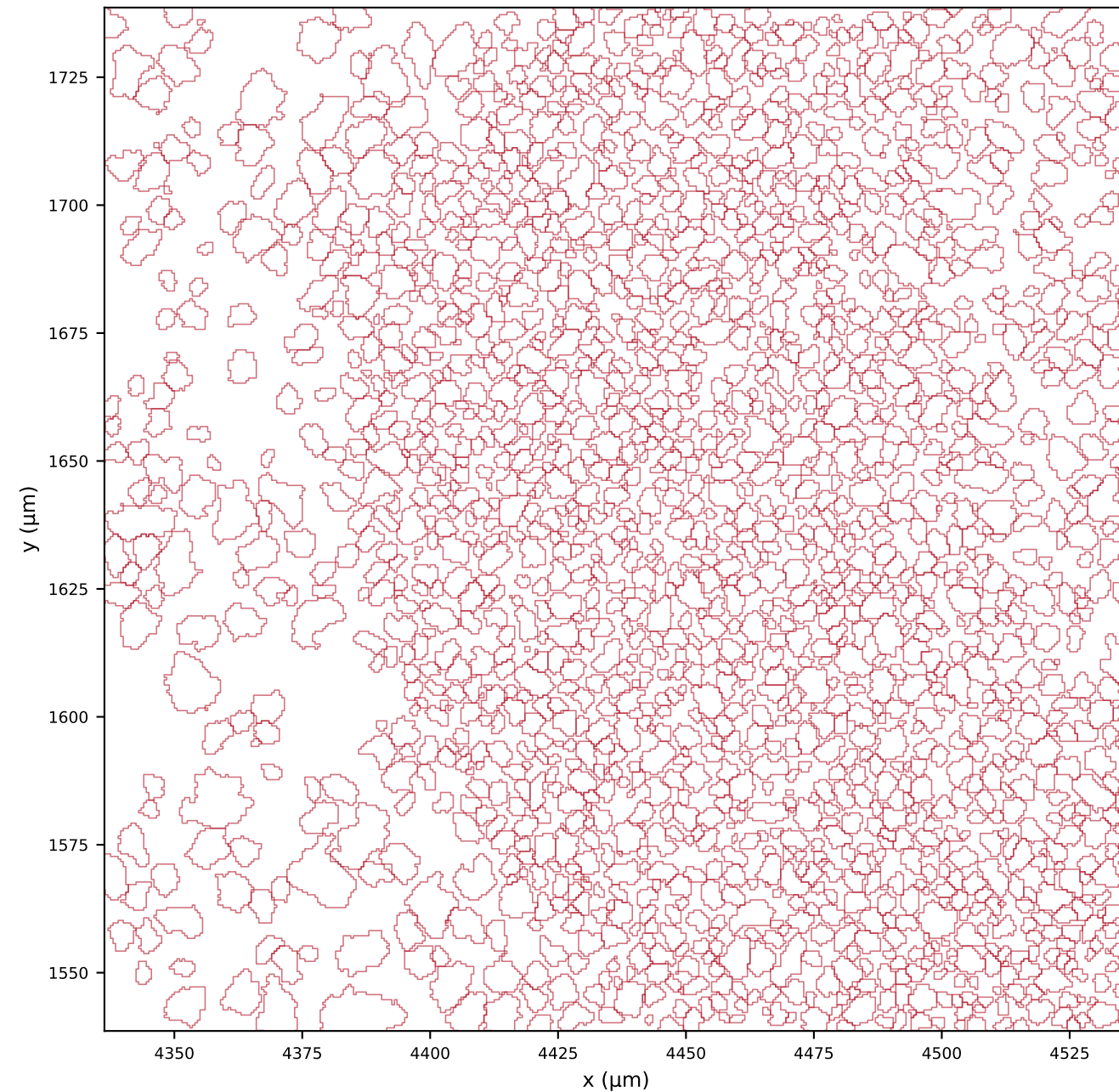
ProSeg (1802 cells)
