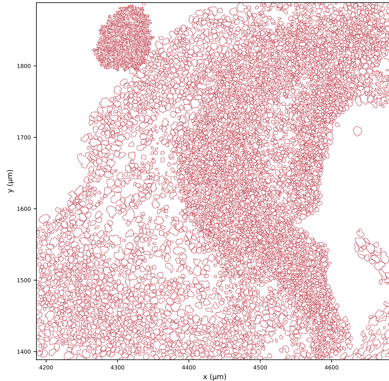
ProSeg (6494 cells)
