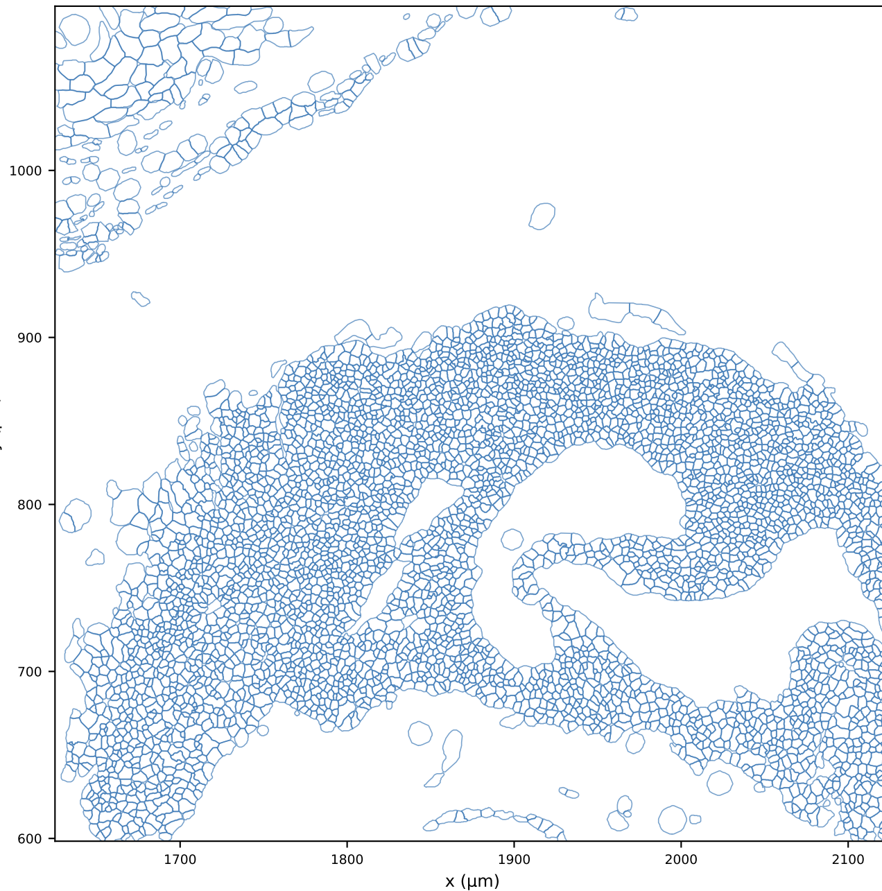
Xenium Original (4746 cells)
