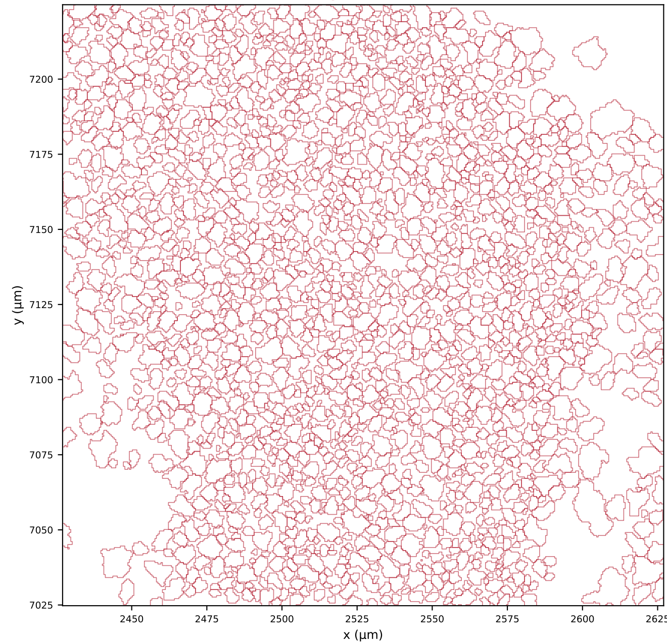
ProSeg (1769 cells)
