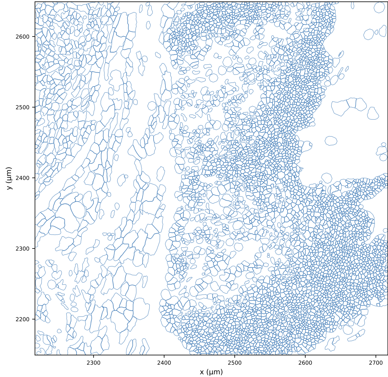
Xenium Original (4892 cells)
