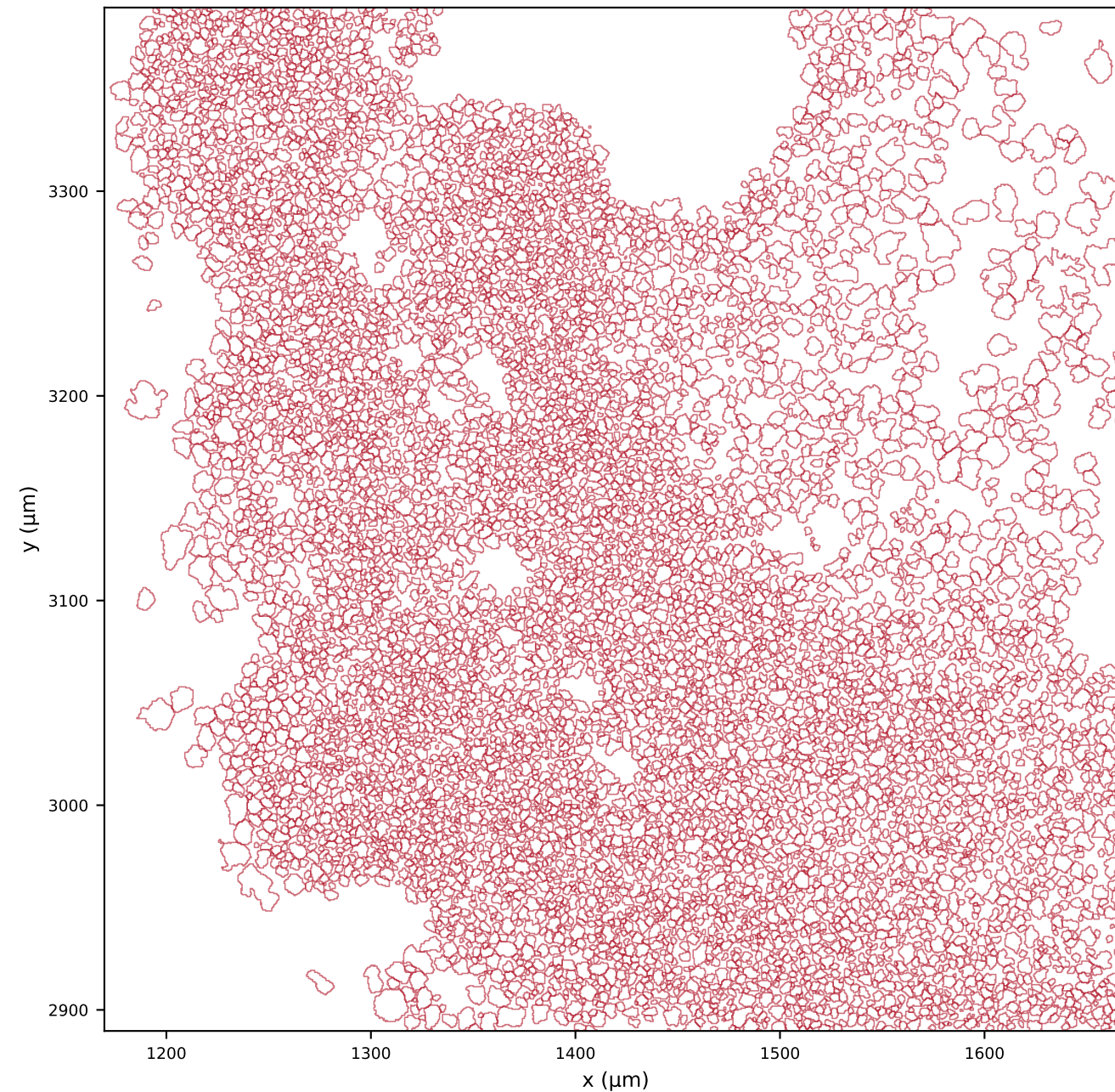
ProSeg (7130 cells)
