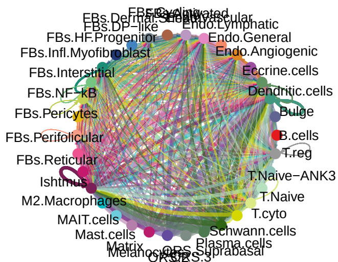
MIF signaling pathway network
