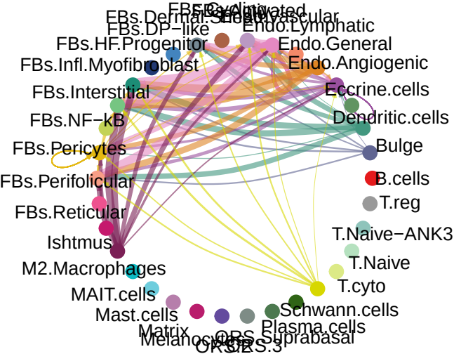
PDGF signaling pathway network
