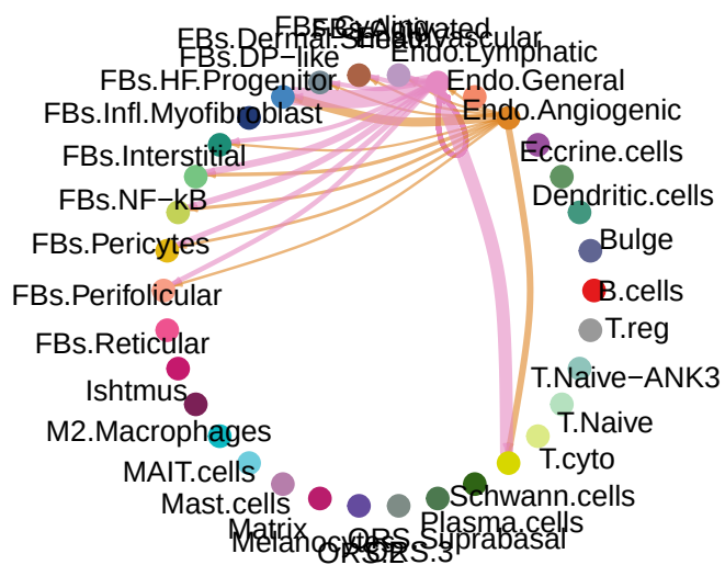
PROS signaling pathway network
