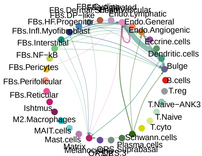
ncWNT signaling pathway network
