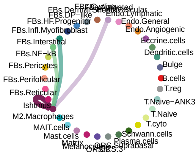
MPLEMENT signaling pathway net
