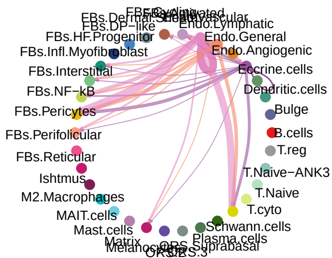
EDN signaling pathway network
