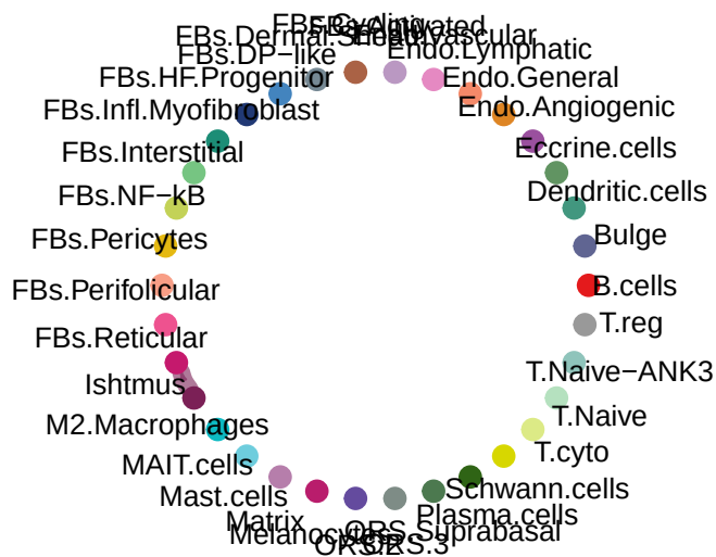
IL1 signaling pathway network
