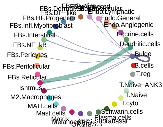
NRG signaling pathway network
