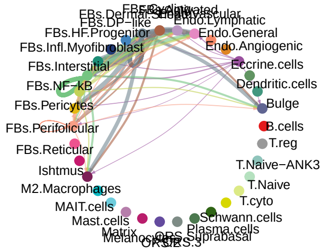
ERIOSTIN signaling pathway netw
