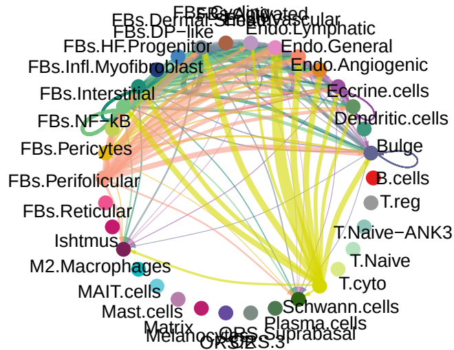
ENASCIN signaling pathway network
