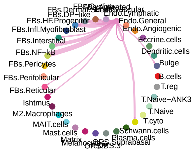
TWEAK signaling pathway network
