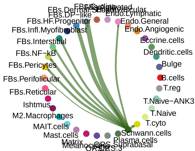
GAS signaling pathway network
