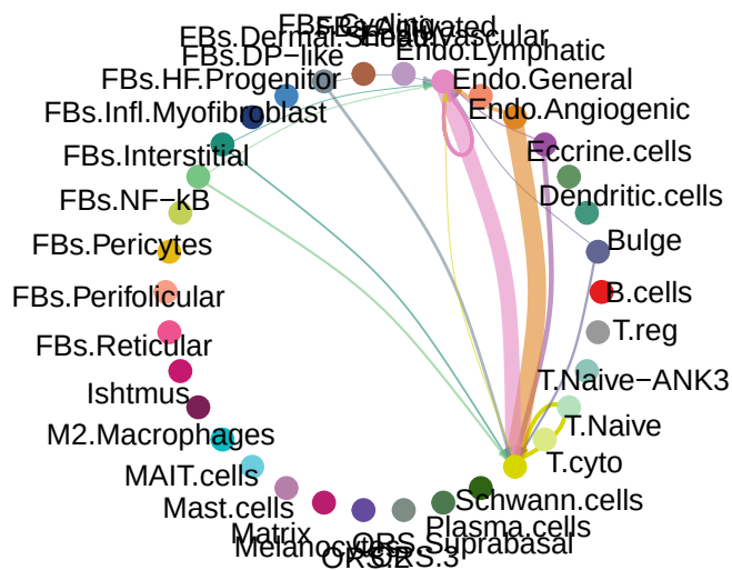
HSPG signaling pathway network
