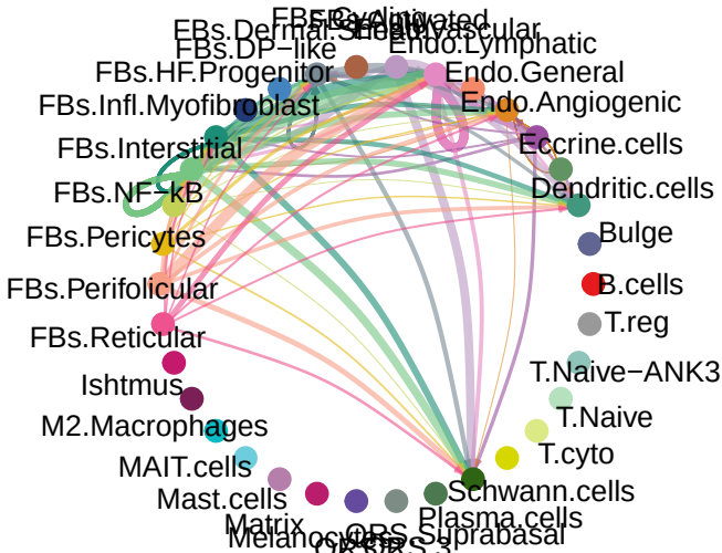
IGFBP signaling pathway network
