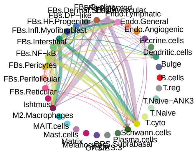
IL6 signaling pathway network
