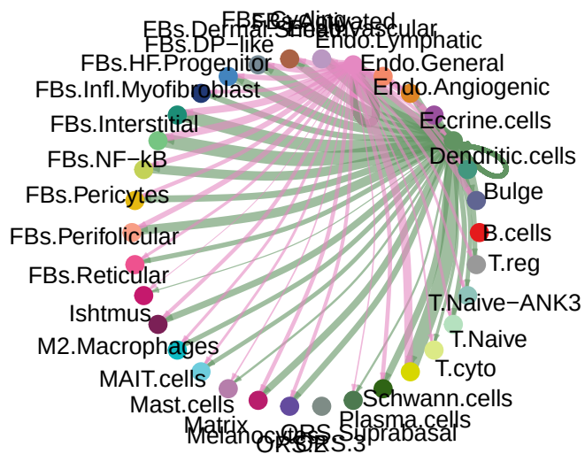
MK signaling pathway network
