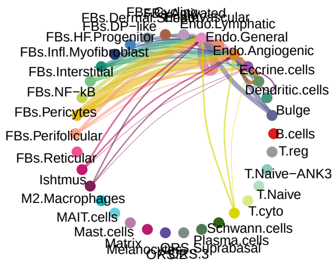
VEGF signaling pathway network
