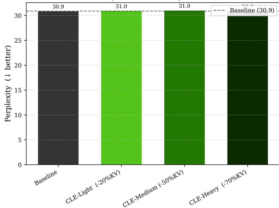
Cross-Layer KV Eviction — Perplexity on PG-19 (Pythia-70M, training-free)
