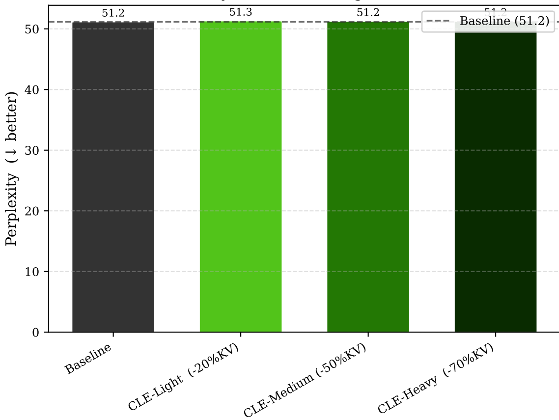
Cross-Layer KV Eviction — Perplexity on WikiText-2 (Pythia-70M, training-free)
