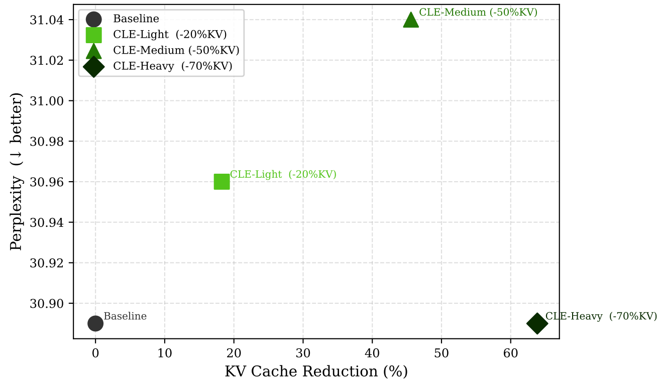
Quality-Memory Tradeoff — PG-19 (Pythia-70M, ctx=1024)
