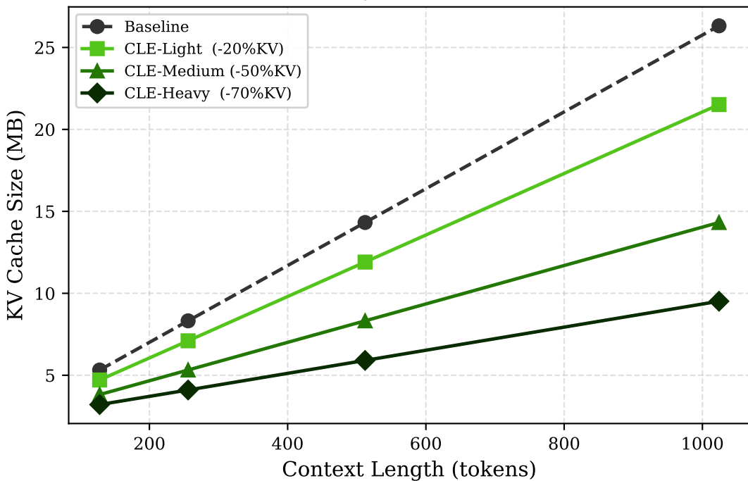
KV Cache Memory vs. Context Length (Pythia-70M)
