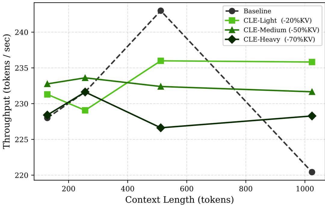
Generation Throughput vs. Context Length (Pythia-70M)
