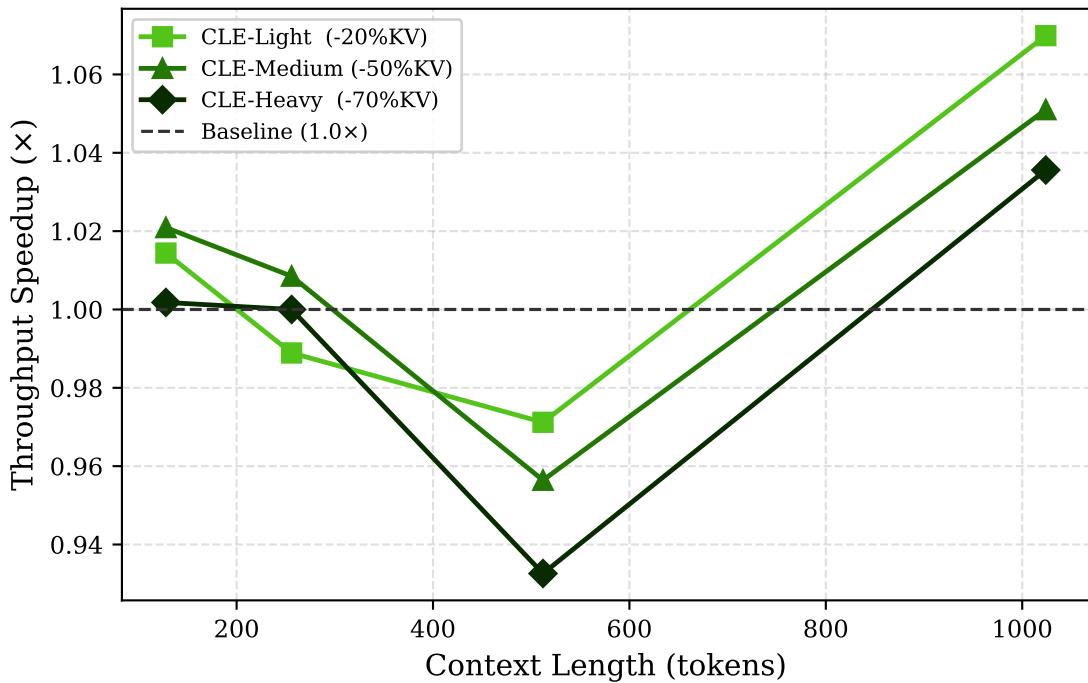
Throughput Speedup vs. Context Length (Pythia-70M)
