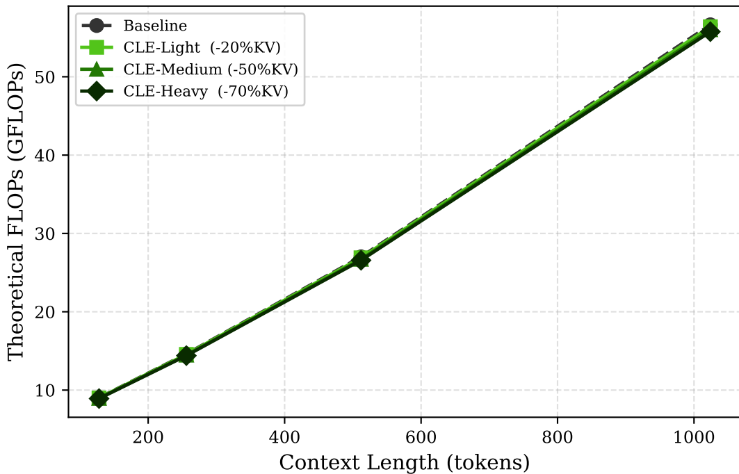
Theoretical FLOPs vs. Context Length (Pythia-70M, analytical)
