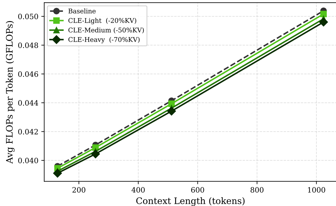
Average FLOPs per Token vs. Context Length (Pythia-70M, analytical)
