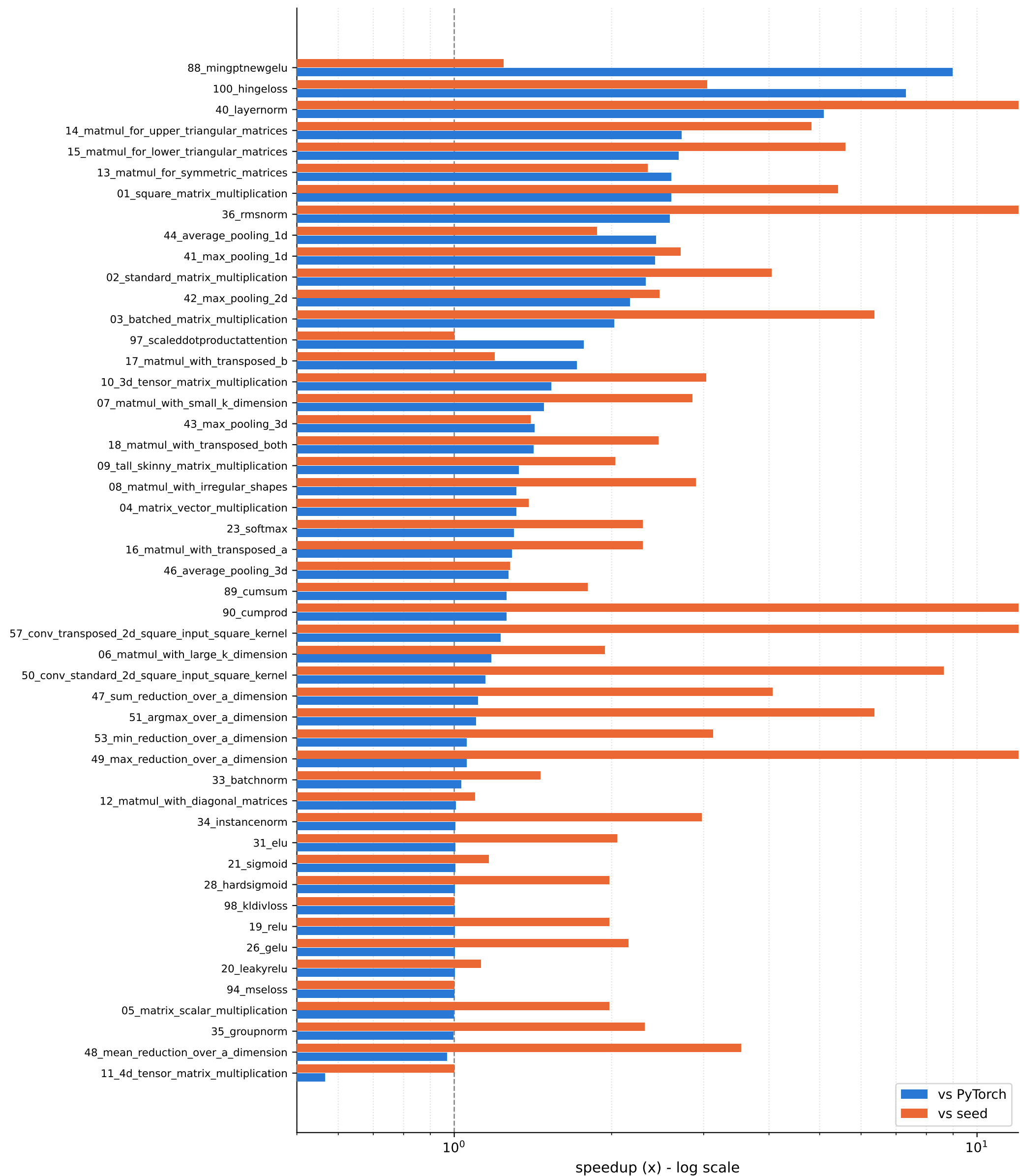
DirectTune-MCTS L1 kernel speedups (49 problems, sorted by vs-PyTorch)
