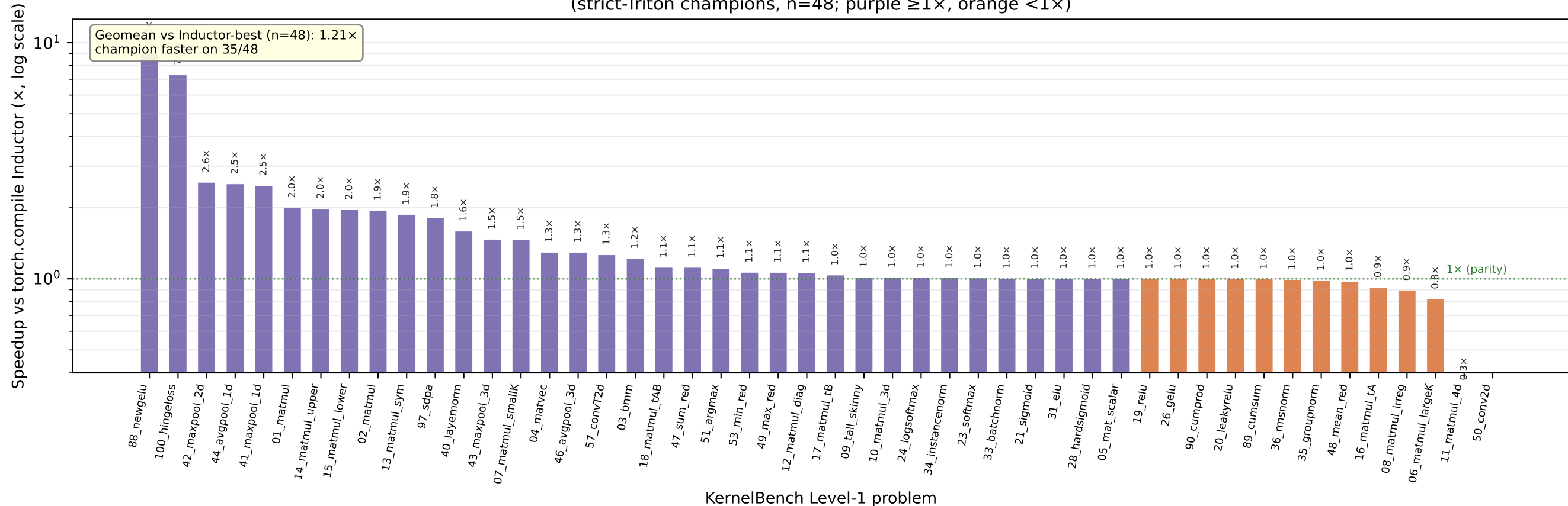
DirecTune-MCTS Level-1: champion speedup vs torch.compile (Inductor, best mode) (strict-Triton champions, n=48; purple \geq 1\times , orange < 1\times )
