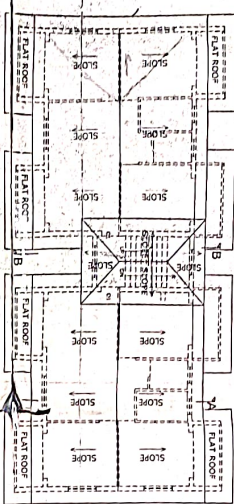
ROOF PLAN
