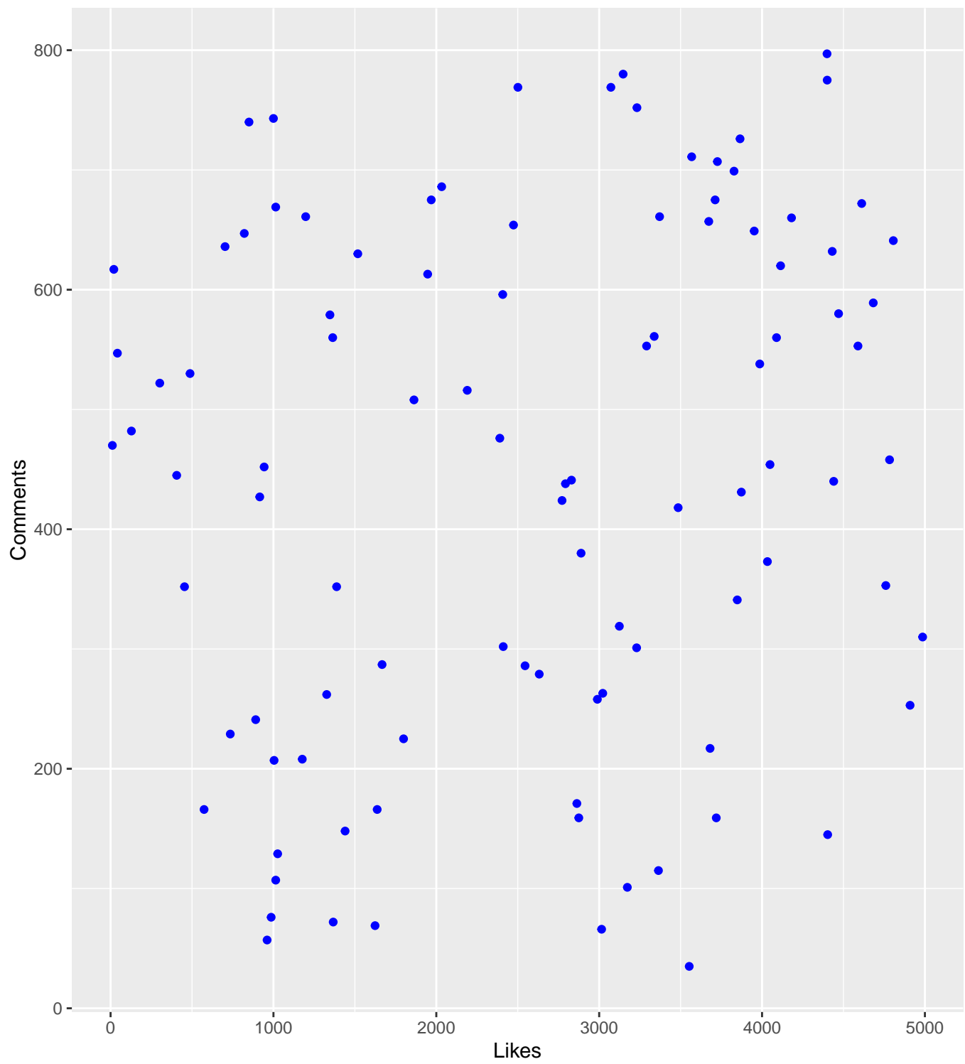
Overplotting Problem
