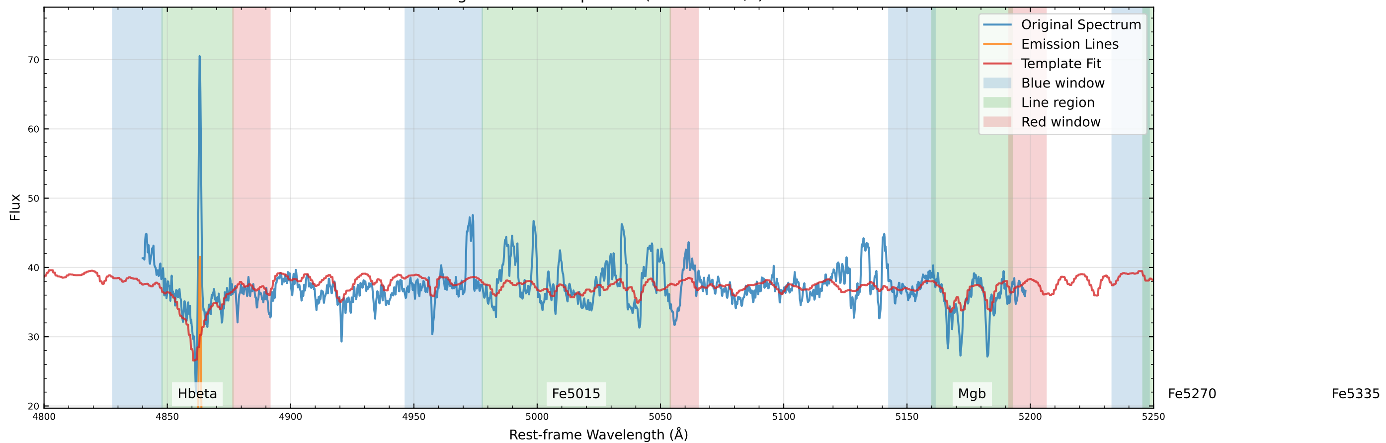
Original Data Comparison ( v=-30.7 km/s)
