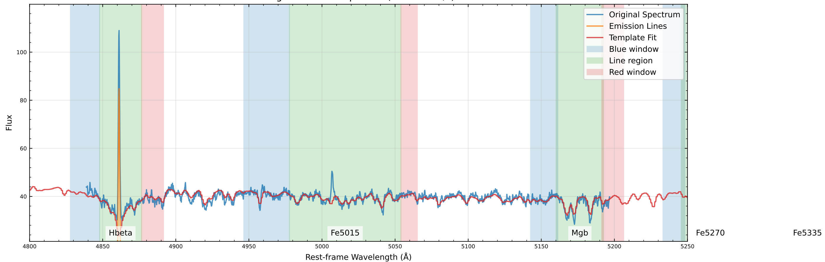
Original Data Comparison (v=41.3 km/s)
