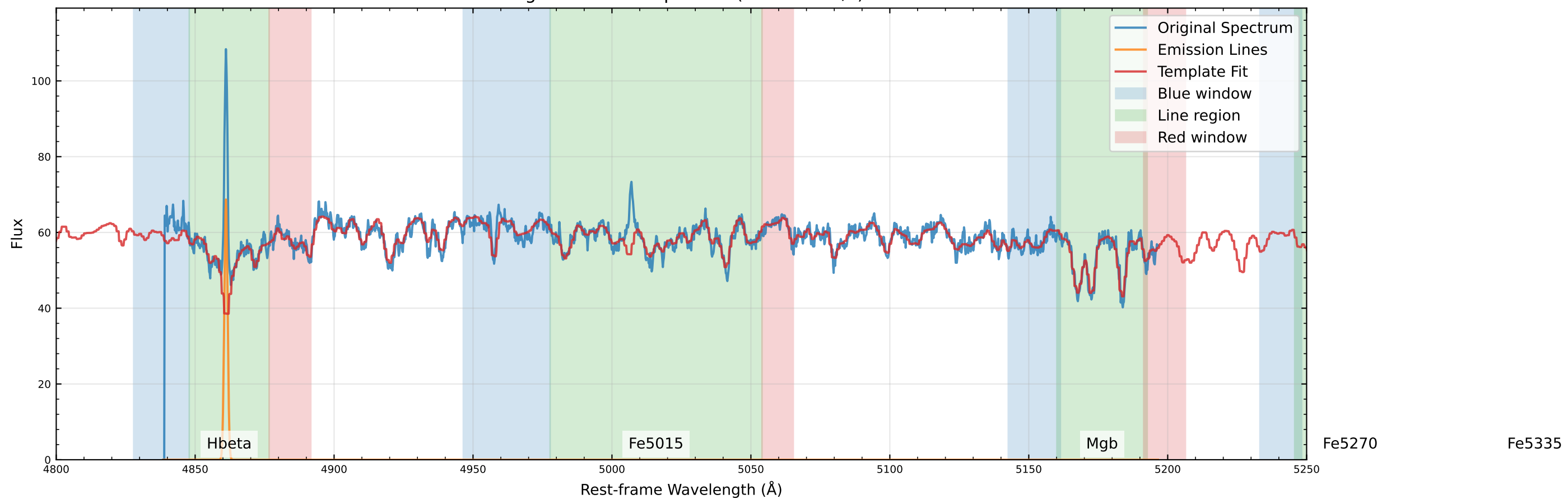
Original Data Comparison (v=60.2 km/s)
