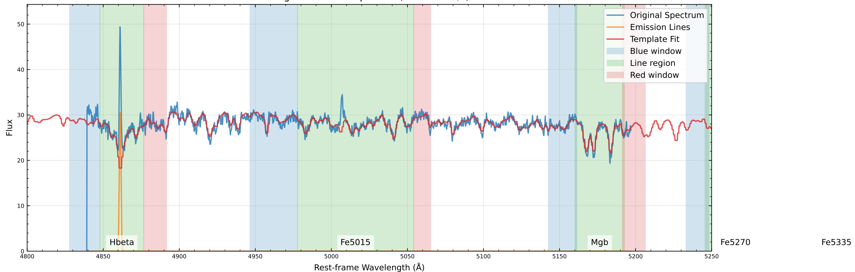
Original Data Comparison (v=29.6 km/s)
