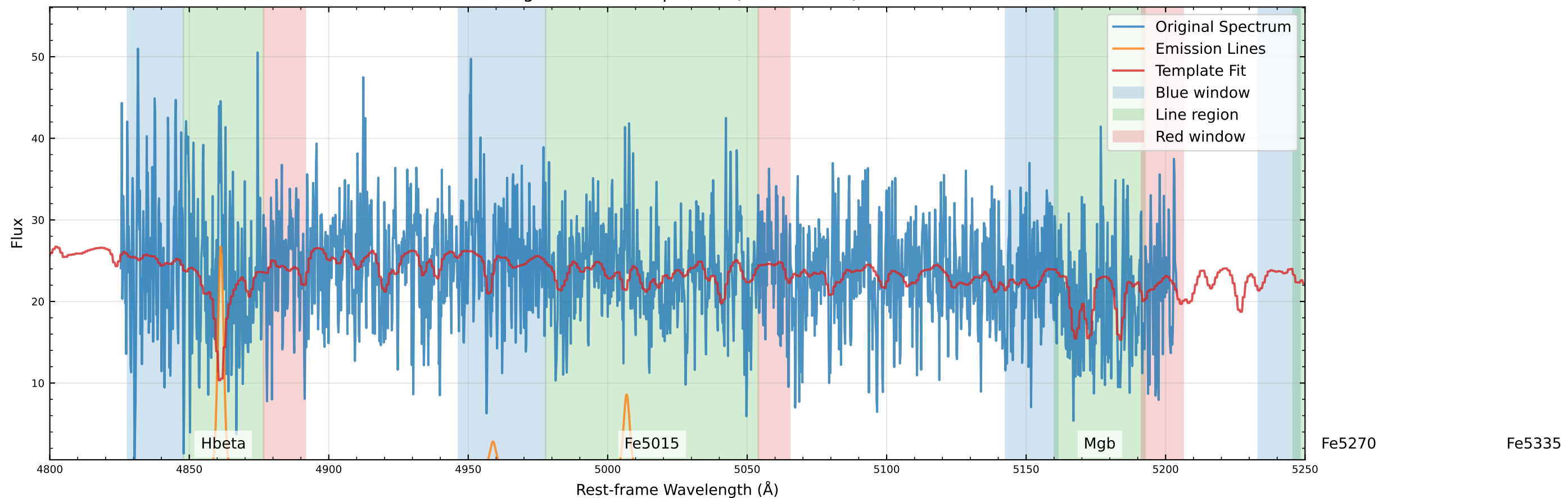
Original Data Comparison (v=-2.4 km/s)
