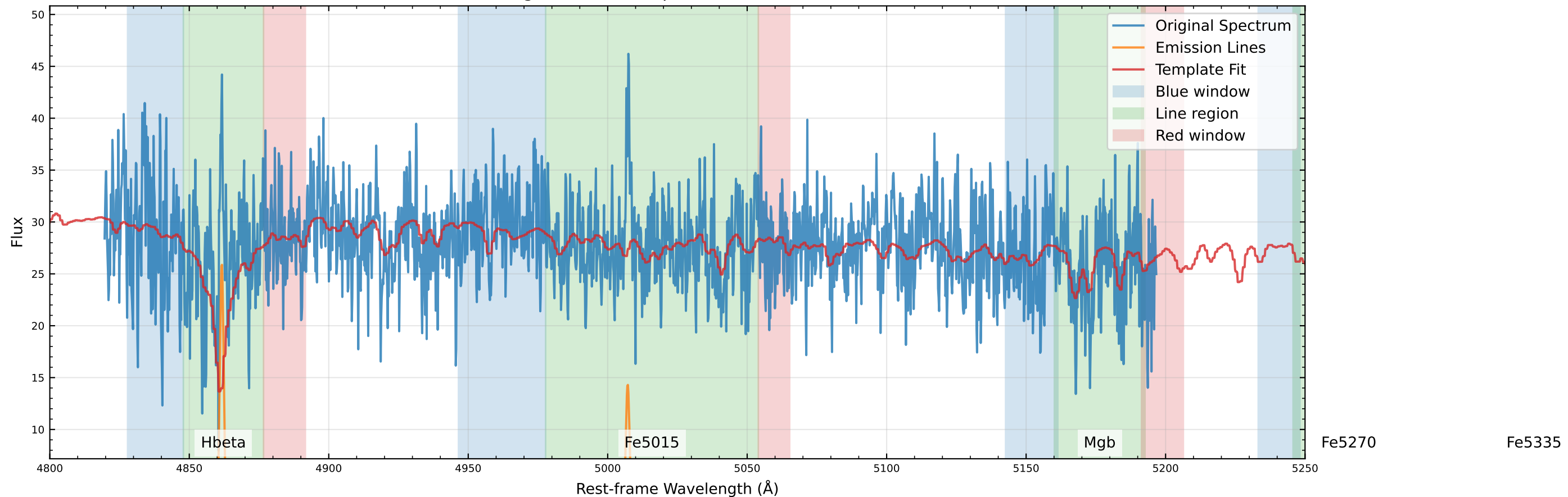
Original Data Comparison (v=-1.0 km/s)
